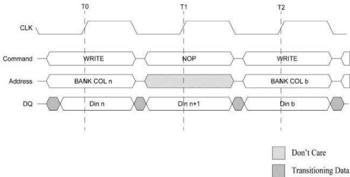
Figure 18: WRITE-TO-WRITE
