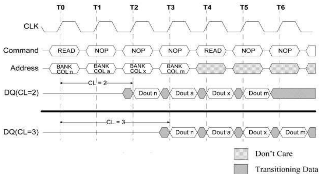
Figure 11: Random READ Accesses
