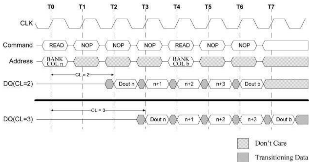
Figure 10: Consecutive READ Bursts
