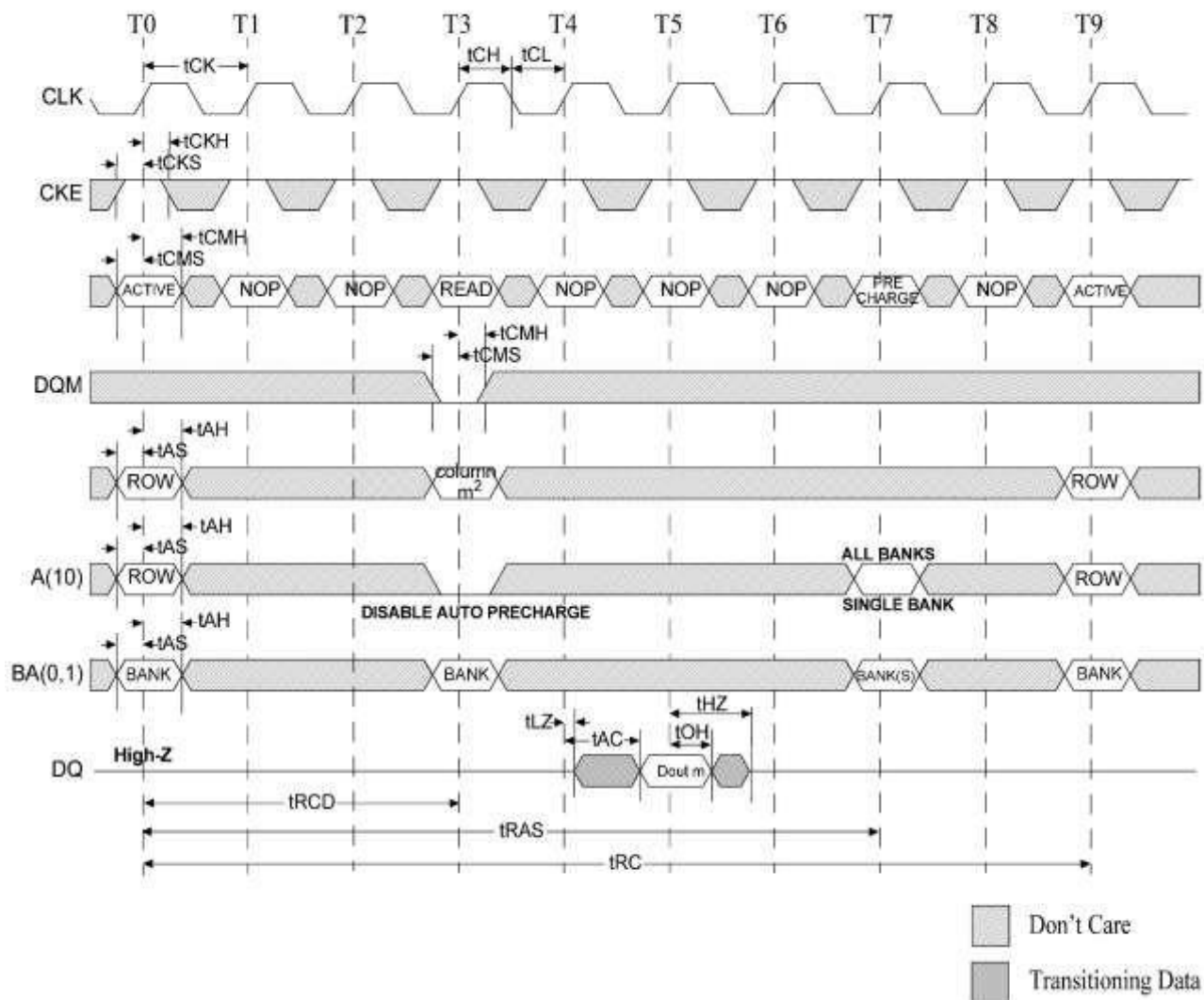
Figure 37: Single READ - Without Auto Precharge
