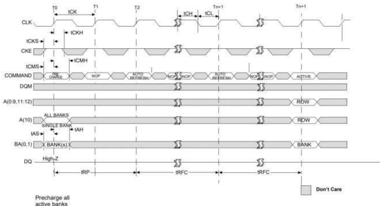
Figure 34: Auto-Refresh Mode
