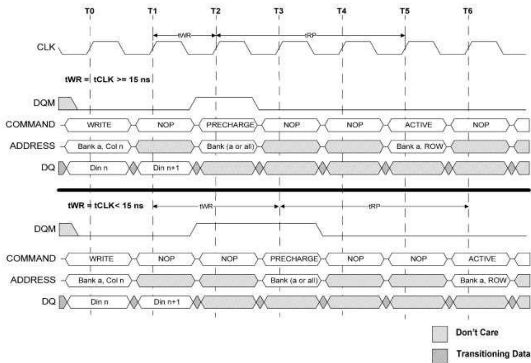
Figure 21: WRITE-to-PRECHARGE
