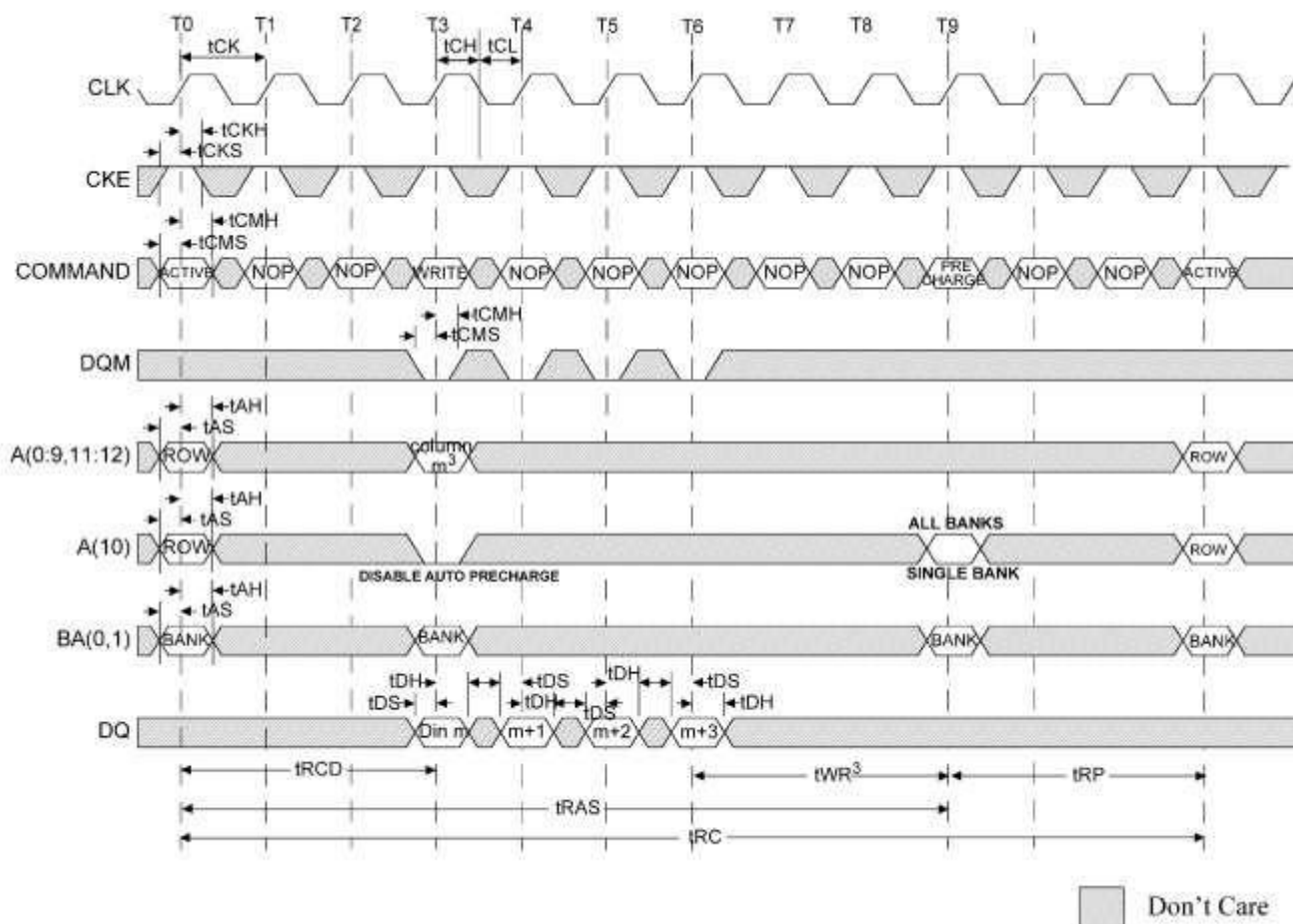
Figure 42: WRITE - Without Auto Precharge
