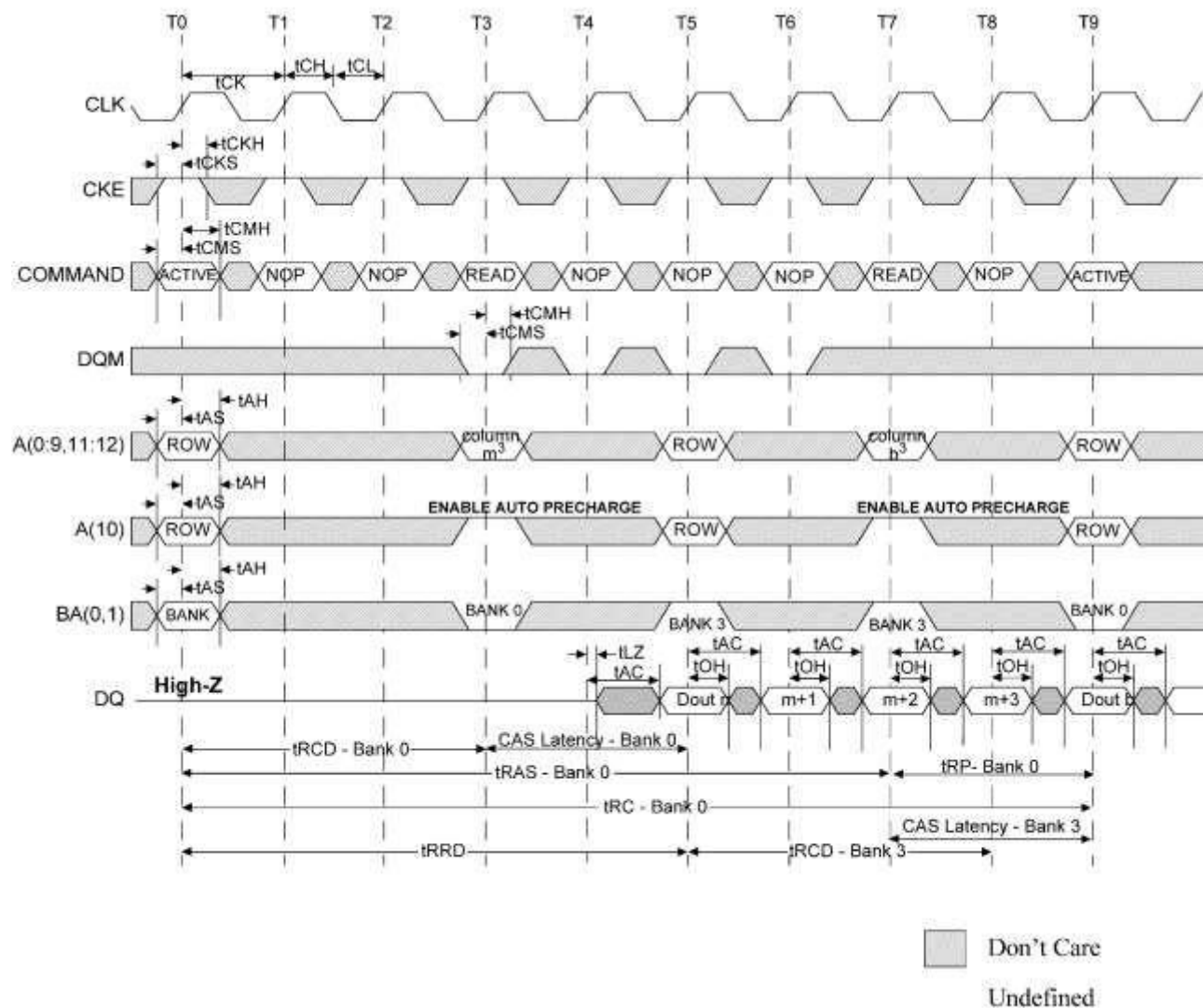
Figure 39: Alternating Bank Read Accesses
