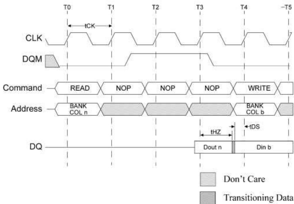
Figure 12: READ-to-WRITE
