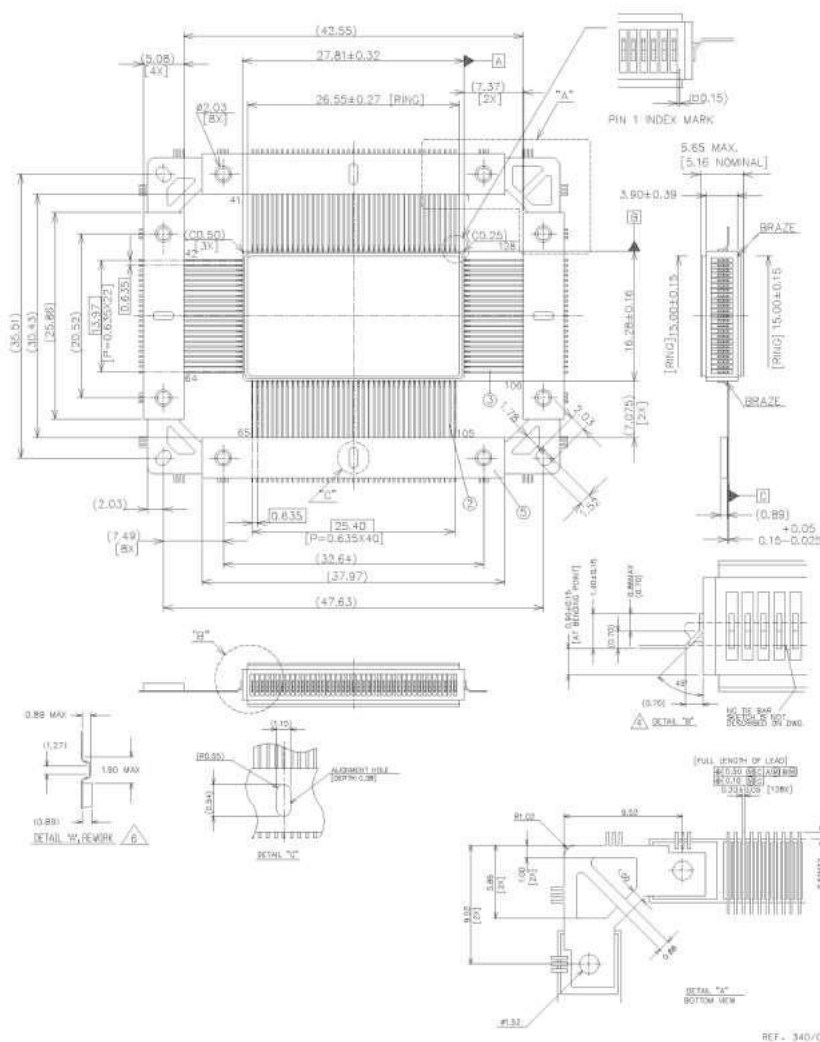
Figure 49: 128-lead Ceramic, Shallow Side-Braze, Dual Sided Quad Flatpack
