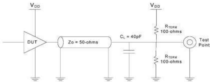
Equivalent Test Load Circuit
