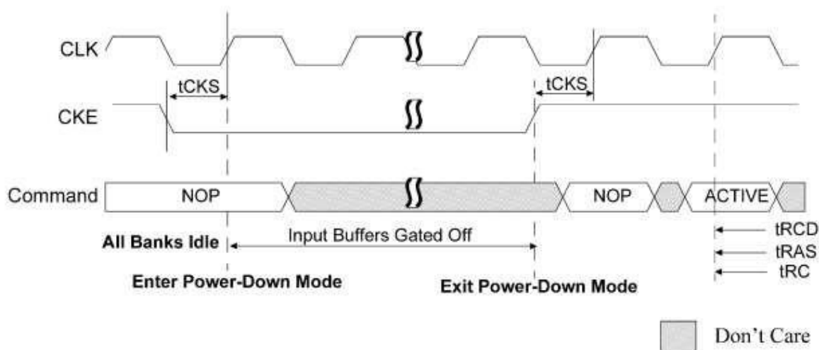
Figure 24: POWER-DOWN
