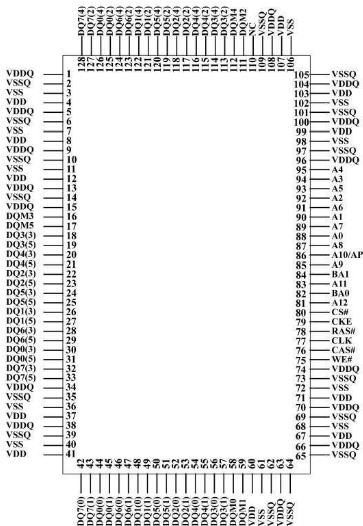
Figure 3: 128-lead Package 3.0G (512Mb x 6) SDRAM Module
