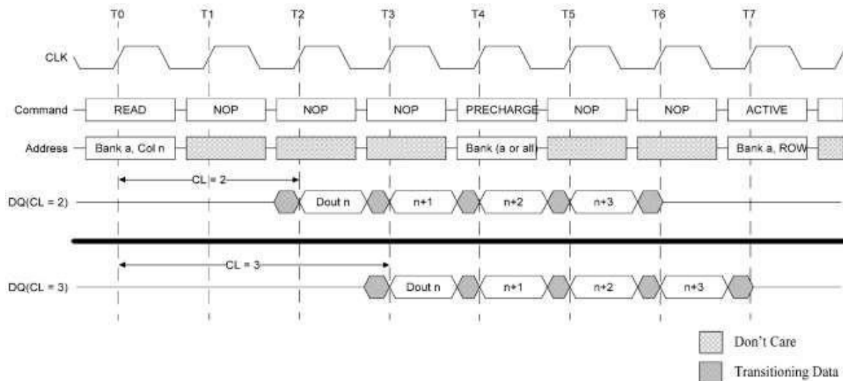
Figure 14: READ-to-PRECHARGE
