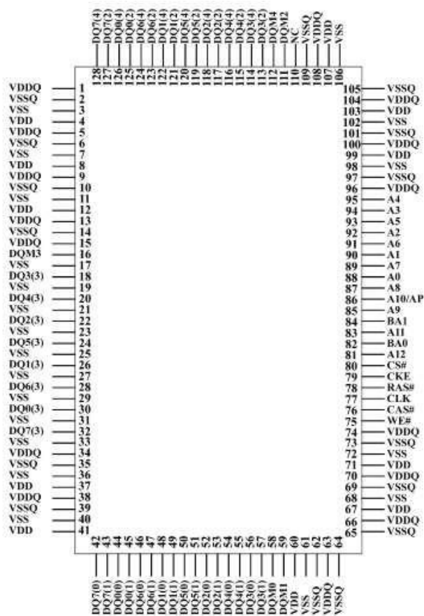
Figure 2: 128-lead Package 2.5G (512Mb x 5) SDRAM Module
