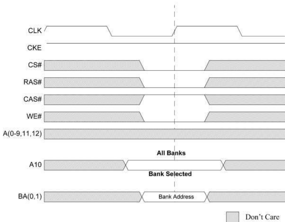
Figure 23: PRECHARGE Command
