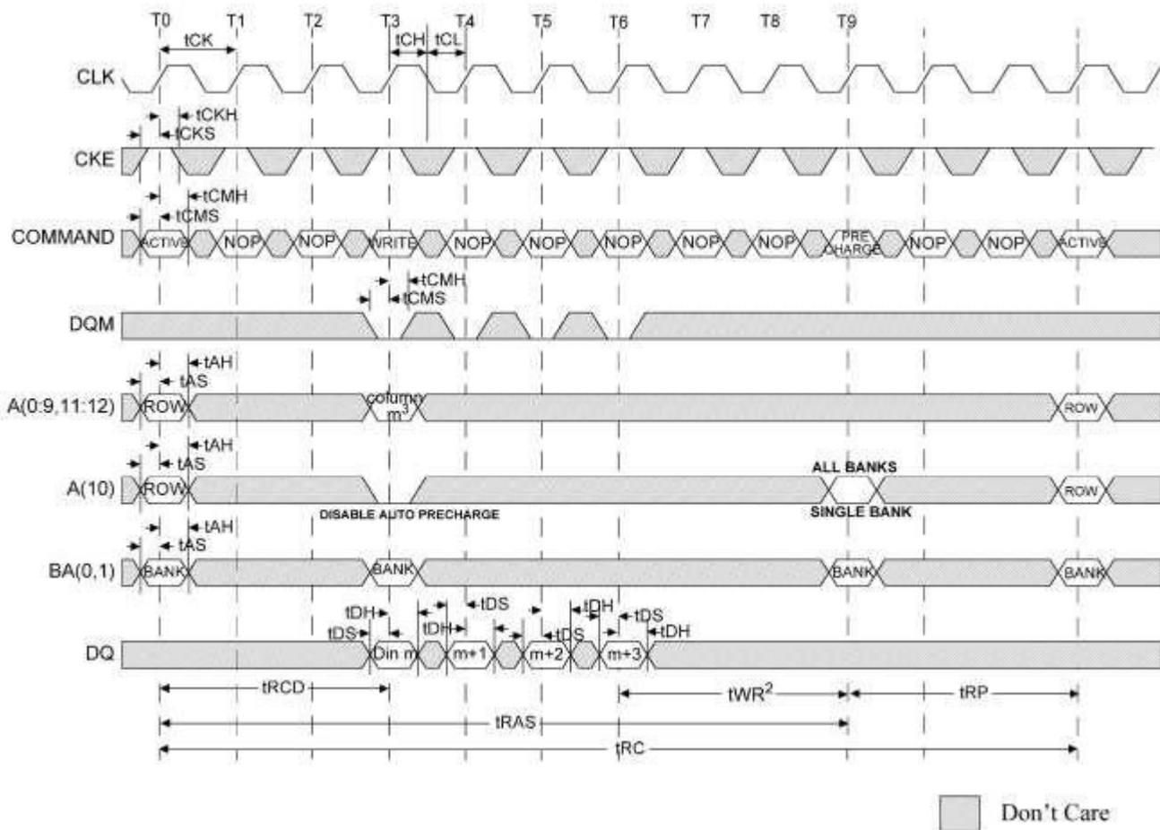
Figure 44: Single WRITE - Without Auto Precharge
