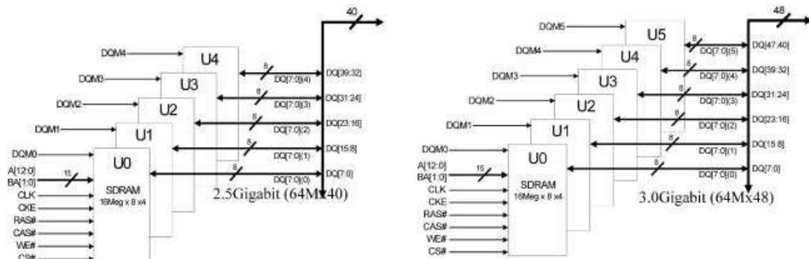
Figure 1. Block Diagrams
