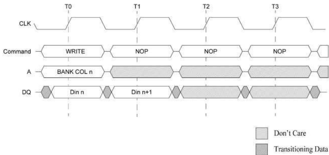
Figure 17: WRITE Burst
