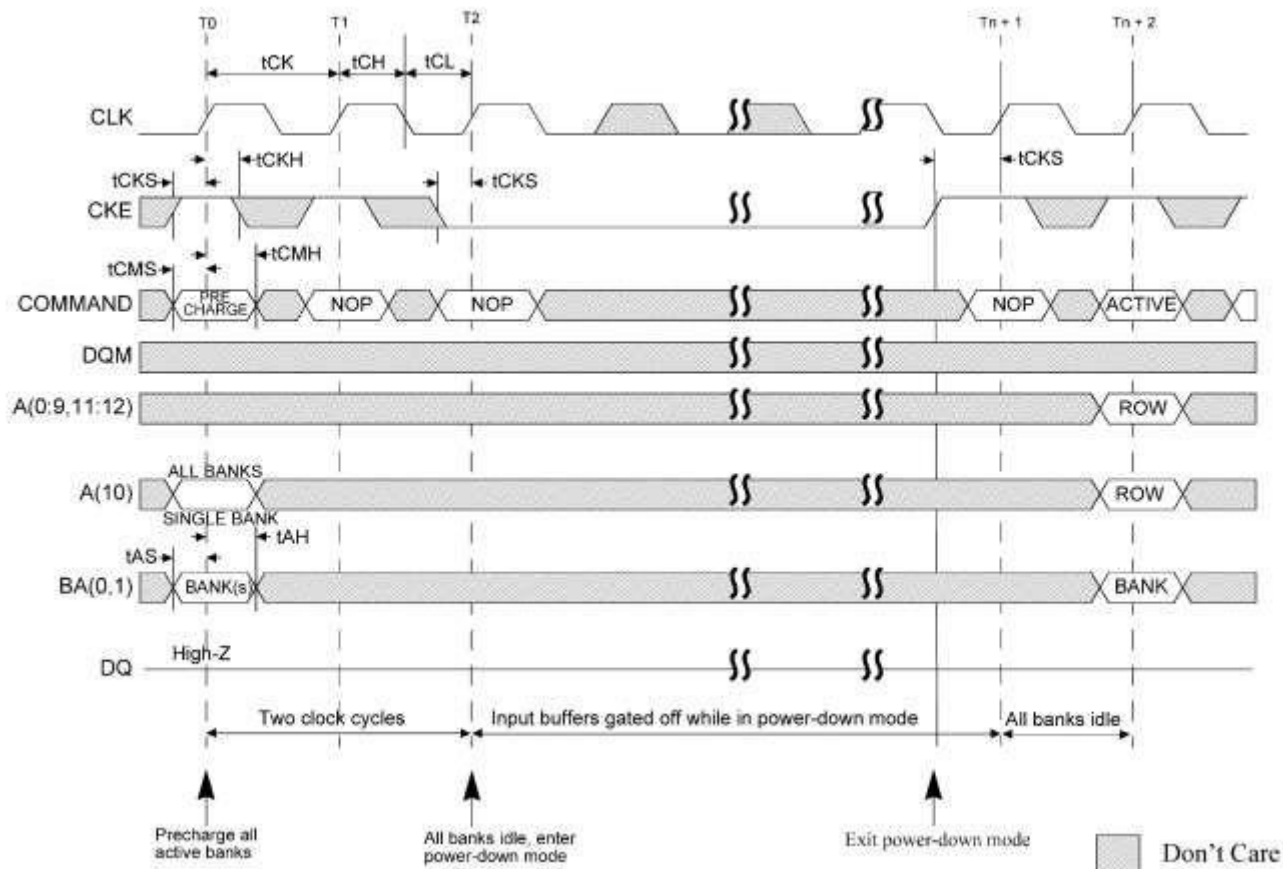
Figure 32: Power-Down Mode
