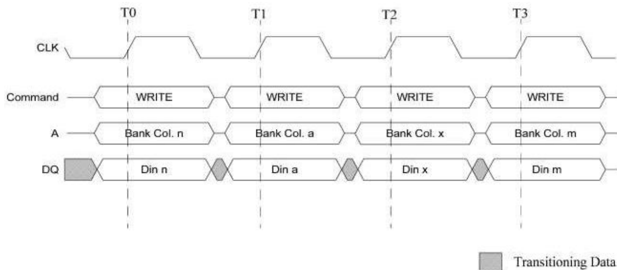
Figure 19: Random WRITE Cycles
