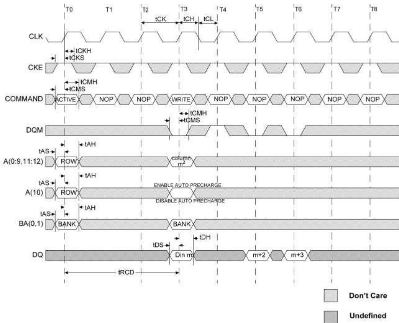
Figure 48: WRITE - DQM Operation
