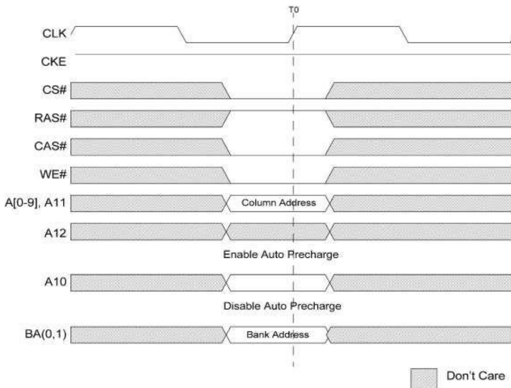
Figure 16: Write Command
