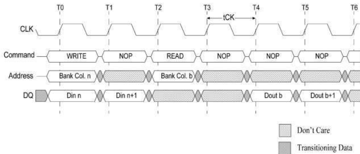
Figure 20: WRITE-to-READ
