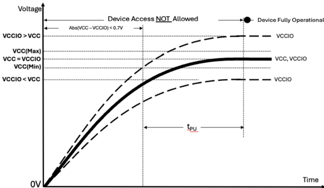
Figure 6: Power-Up Behavior
