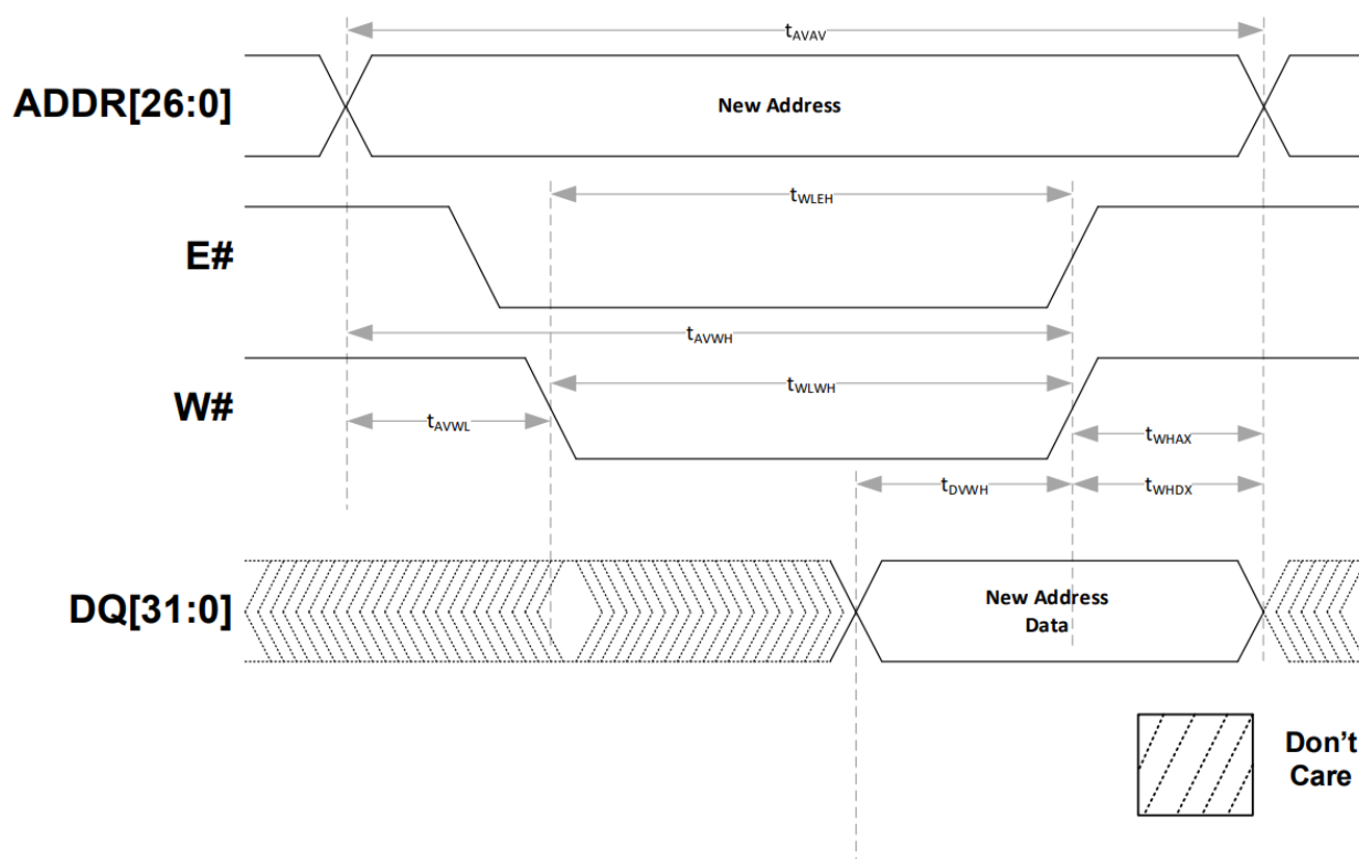
Figure 8: Write Operation (#WE Controlled)
