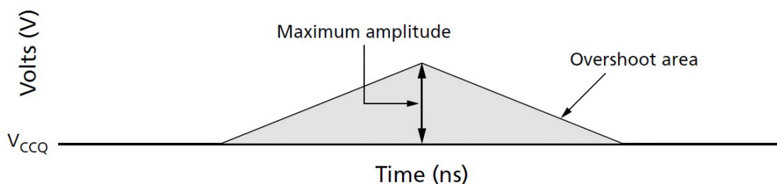
Figure 7: Overshoot
