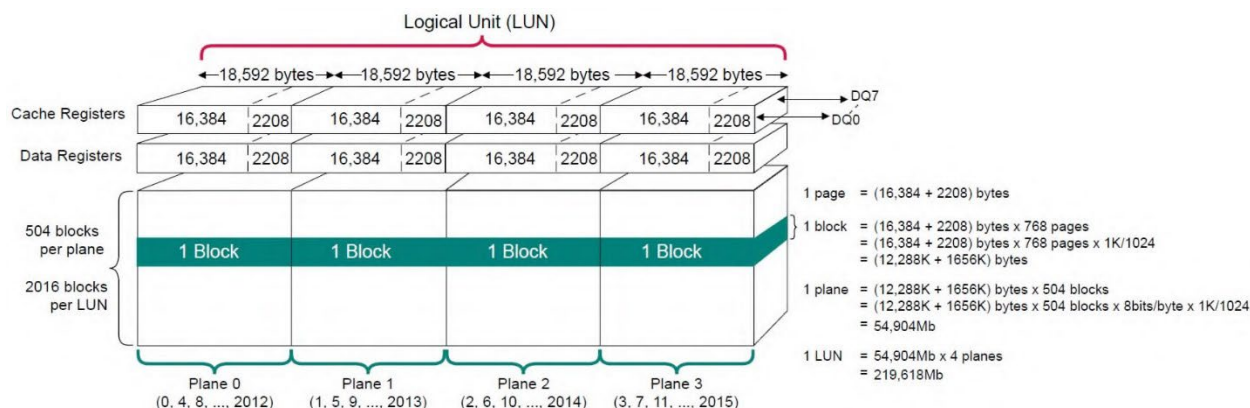
Figure 6: Array Organization per Logical Unit (LUN) in SLC Mode
