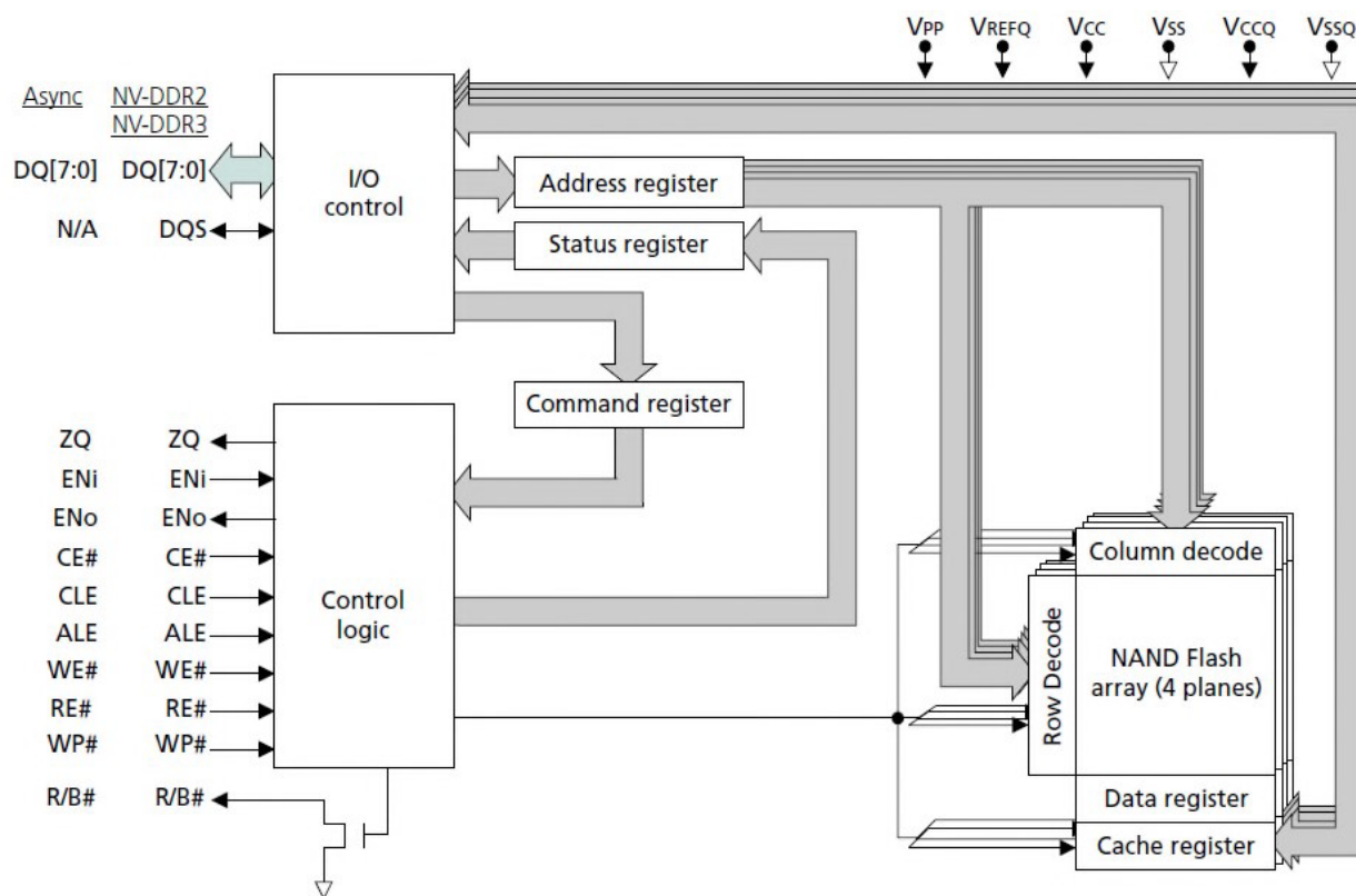
Figure 3: NAND Flash Die (LUN) Functional Block Diagram
