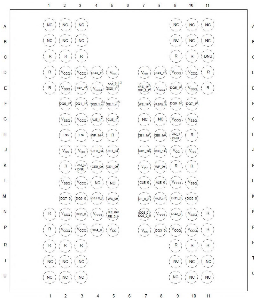
Figure 1: 132-Ball BGA (Ball-Down, Top View)
