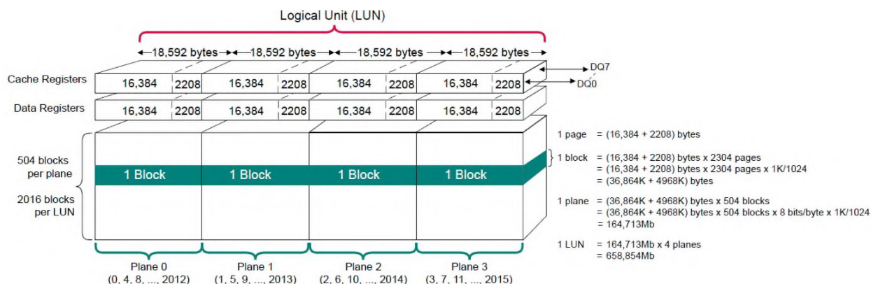
Figure 5: Array Organization per Logical Unit (LUN) in TLC mode
