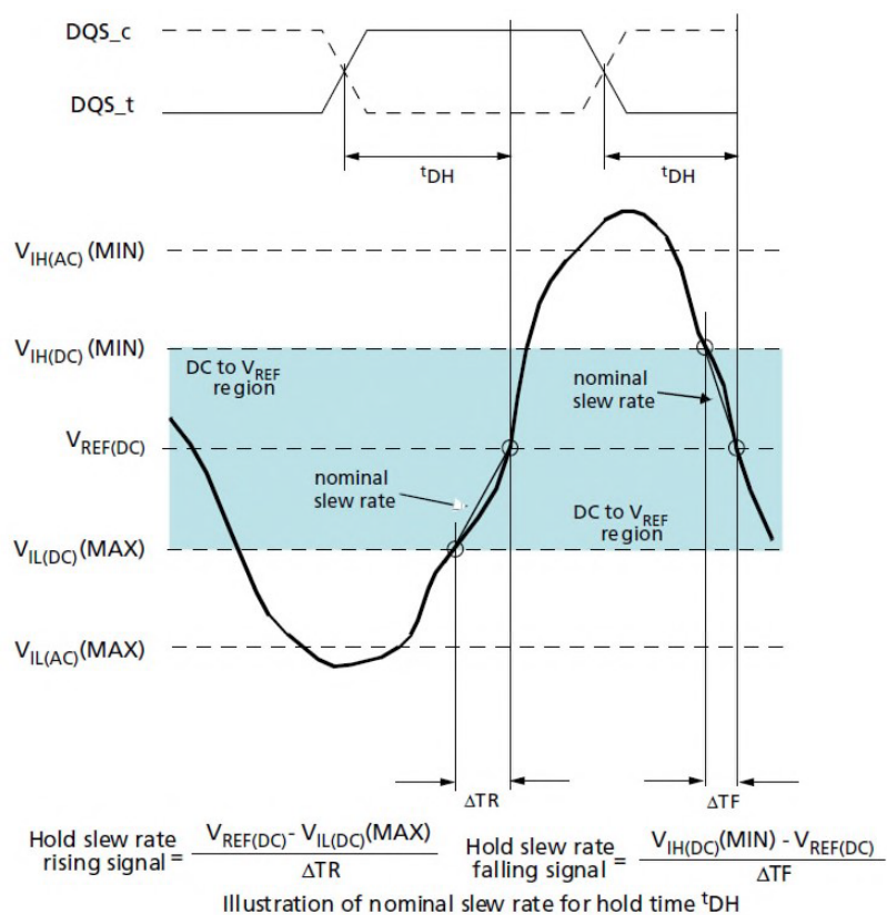
Figure 10: Tangent Line for Data Setup Time ( t_{DS} ), NV-DDR2/NV-DDR3 only
