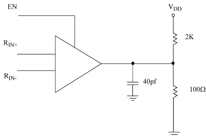
Figure 6. Receiver Three-State Delay Test Circuit or Equivalent Circuit
