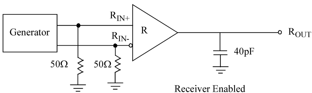
Figure 5. Receiver Propagation Delay and Transition Time Waveforms
