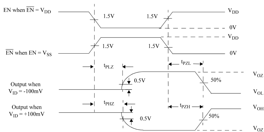
Figure 7. Receiver Three-State Delay Waveform
