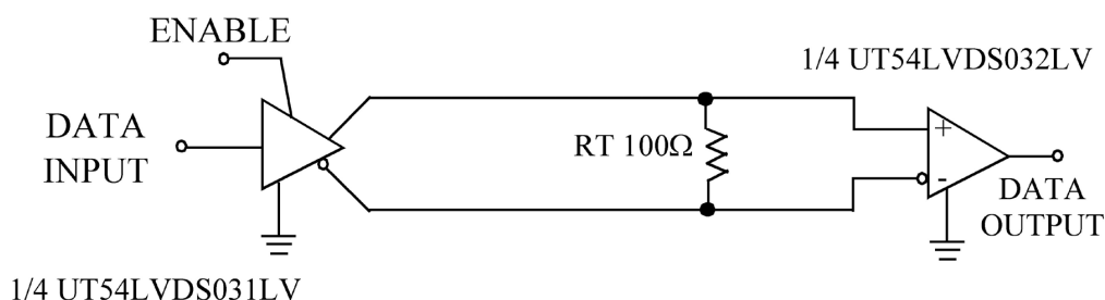
Figure 3. Point-to-Point Application
