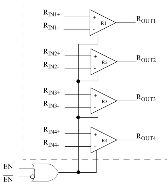
Figure 2. UT54LVDS032LV Pinout
