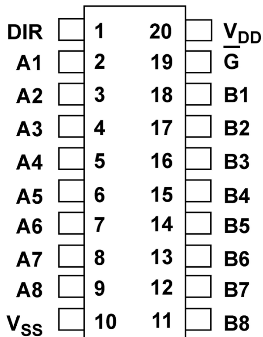
Figure 1: 20-Pin DIP, Top View
