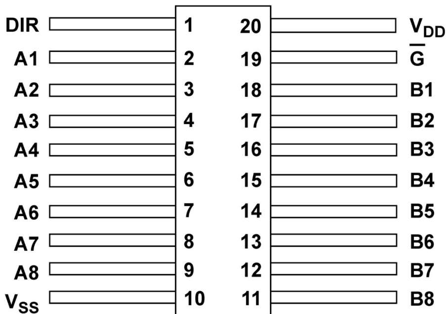
Figure 2: 20-Lead Flatpack, Top View
