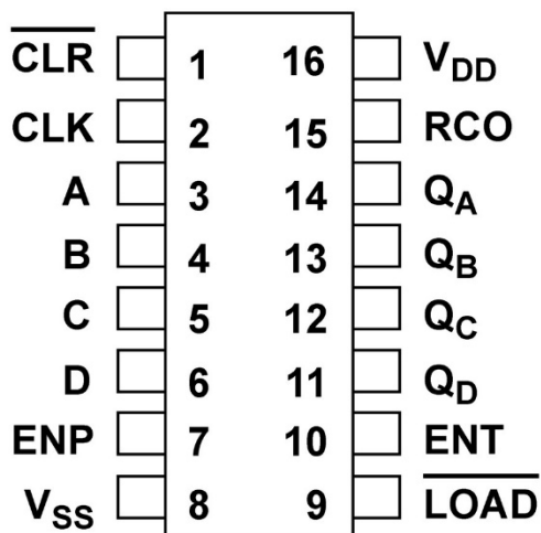
Figure 1: 16-Pin DIP Top View
