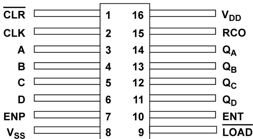
Figure 2: 16-Lead Flatpack Top View
