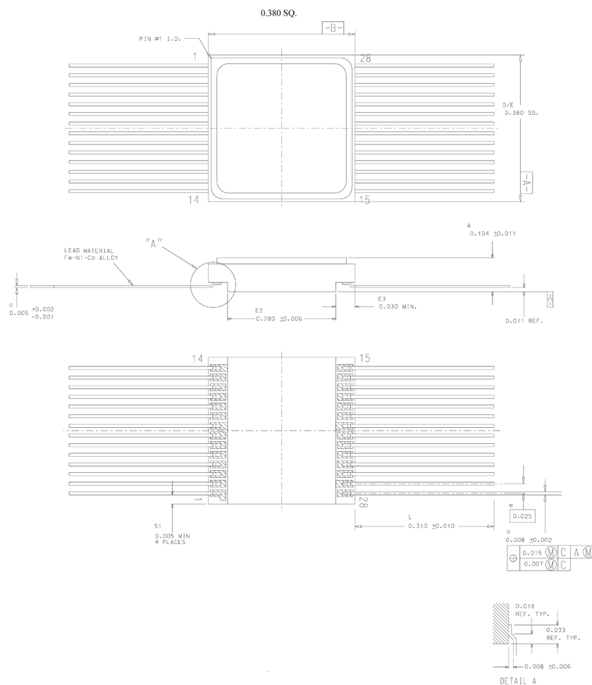
Figure 10: 28-pin Flatpack
