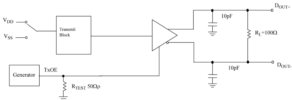
Figure 3: Driver Three-State Delay Time Test or Equivalent Circuit
