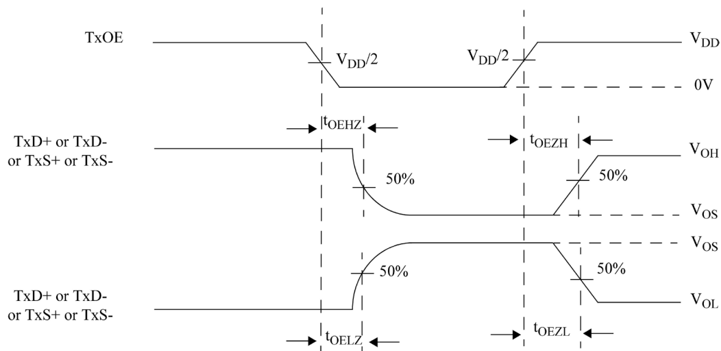
Figure 4: Figure 4. Output Enable to Data Out Timing
