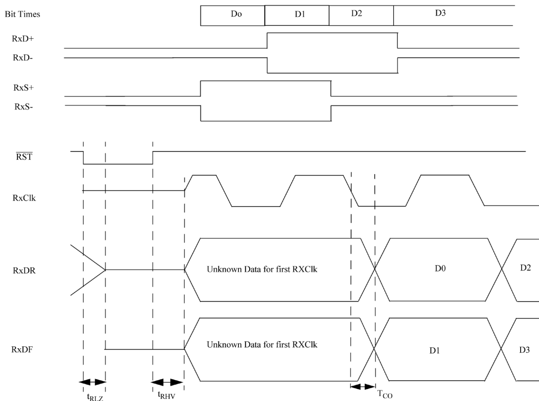
Figure 7: Receiver Output Timing Diagram
