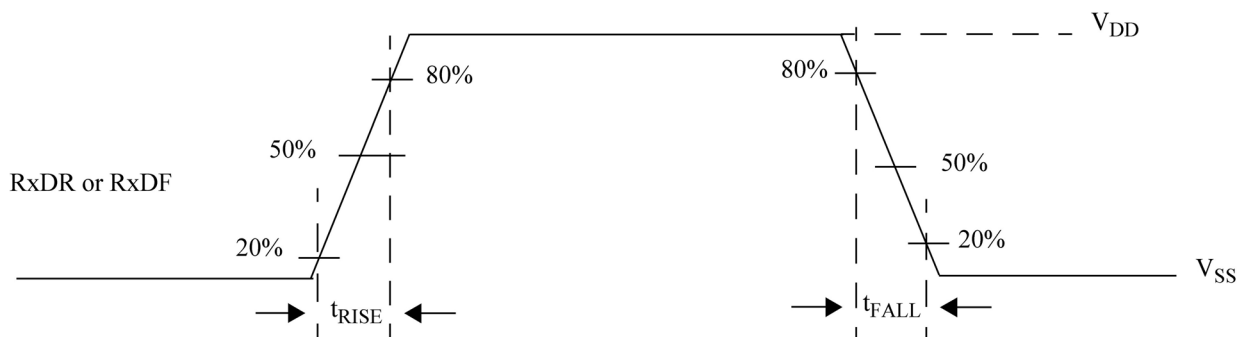
Figure 8: Receiver Output Rise and Fall Times Waveform
