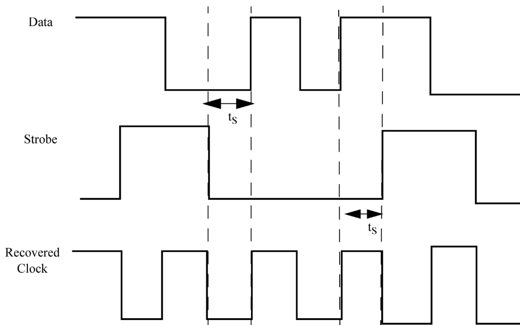
Figure 9: Data/Strobe Separation
