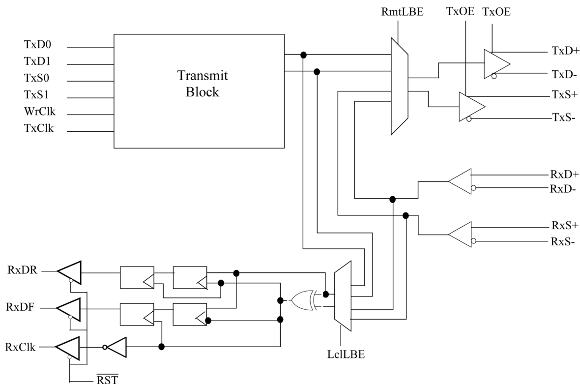
Figure 1: UT200SpWPHY01 SpaceWire PHY Chip Block Diagram
