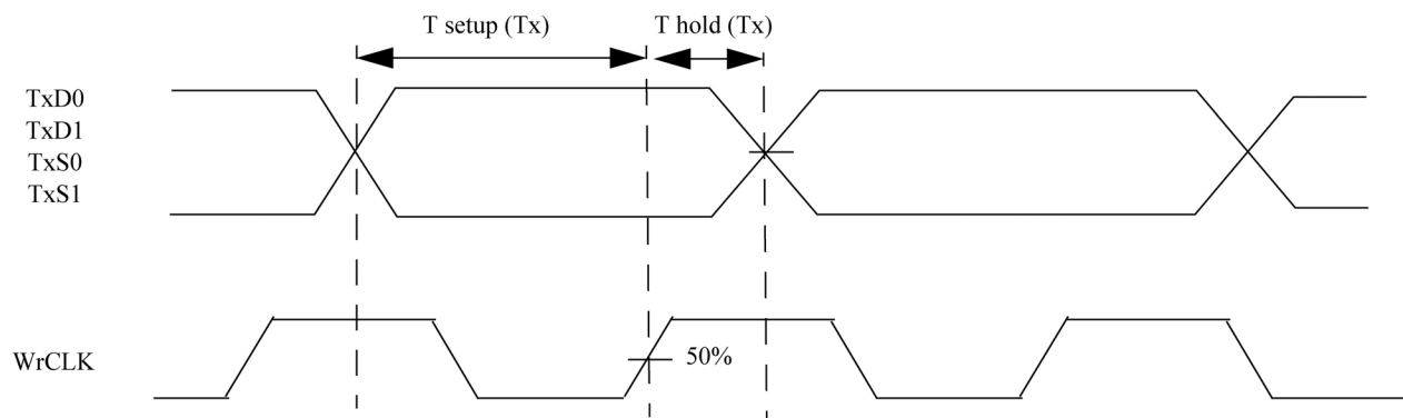
Figure 6: Transmitter Input Timing Diagram
