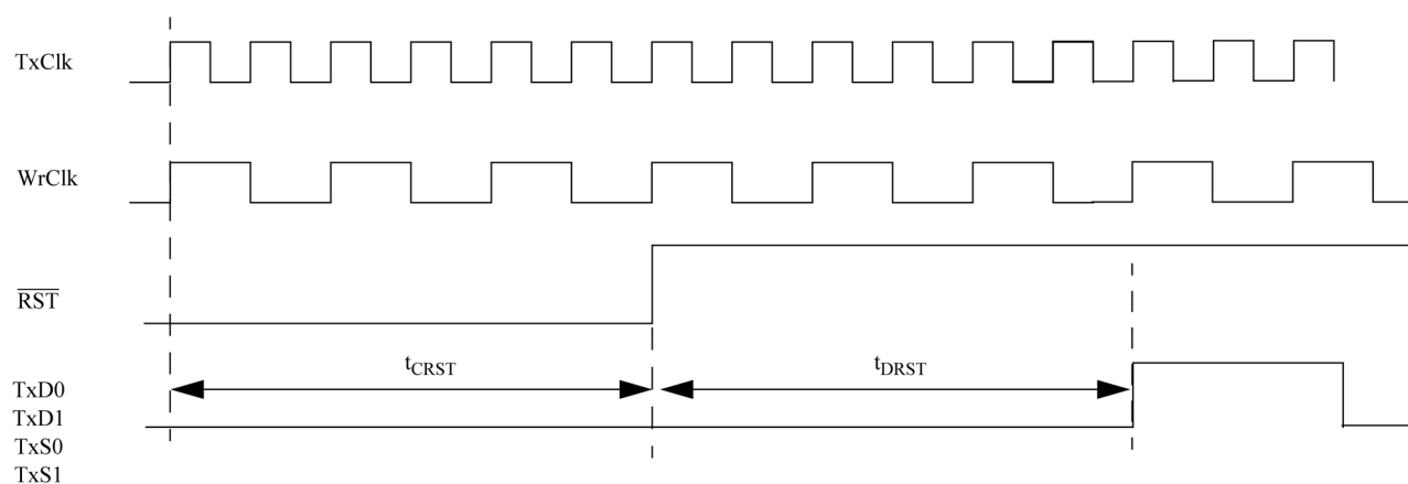
Figure 5: Reset Timing Diagram
