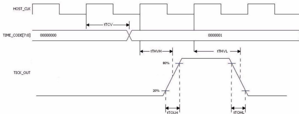
Figure 33: TICK_OUT Interface
