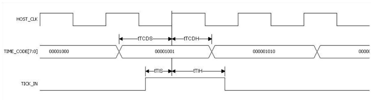
Figure 32: TICK_IN
