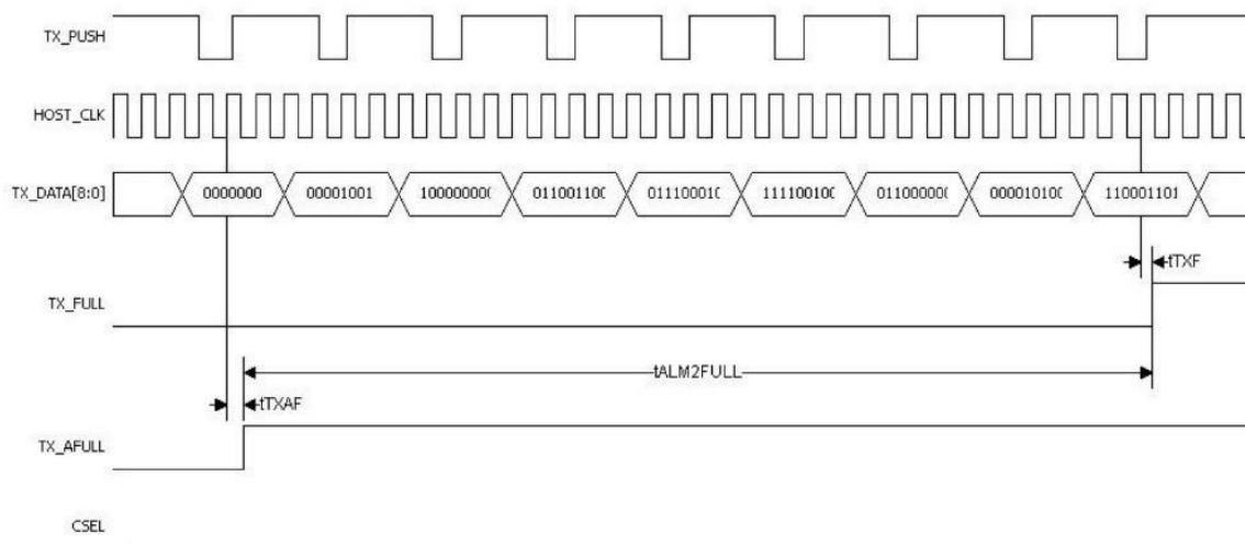
Figure 35: Transmit FIFO Almost Full Flag
