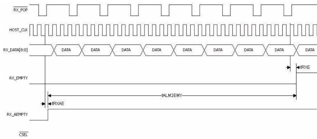
Figure 38: Receive FIFO Almost Empty Flag
