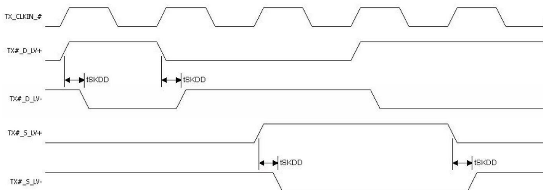
Figure 23: LVDS Driver tSKDD Timing Diagram
