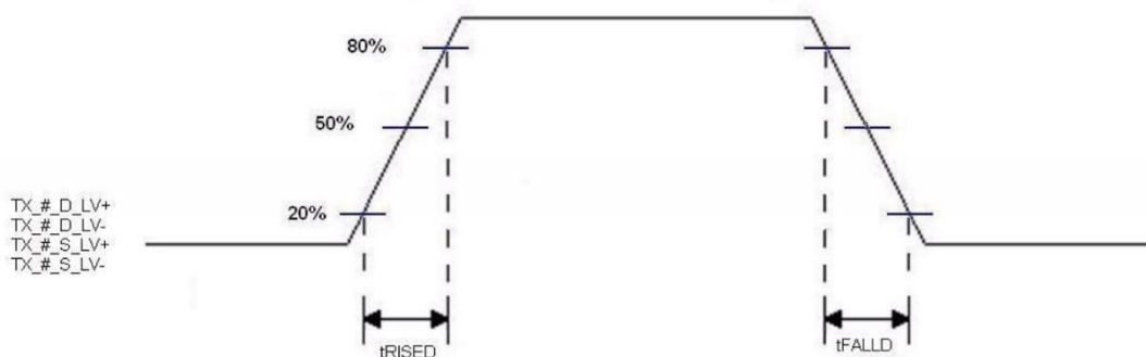
Figure 24: LVDS Driver Rise and Fall Timing Diagram
