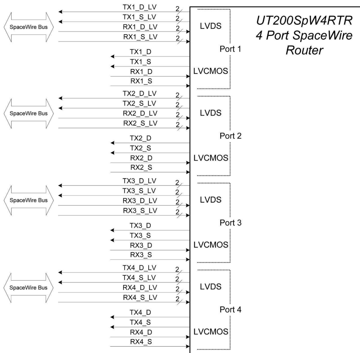
Figure 4:4-Port Router External LVDS Interface
