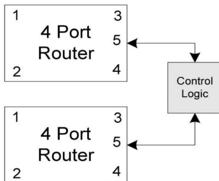
Figure 15: 8-Port Extended Configuration using External Logic
