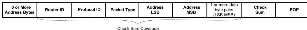
Figure 12: Configuration Port Read Packet Response
