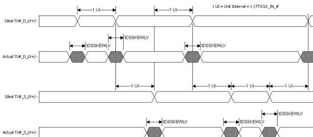
Figure 25: LVDS Driver Data/Strobe Output Skew
