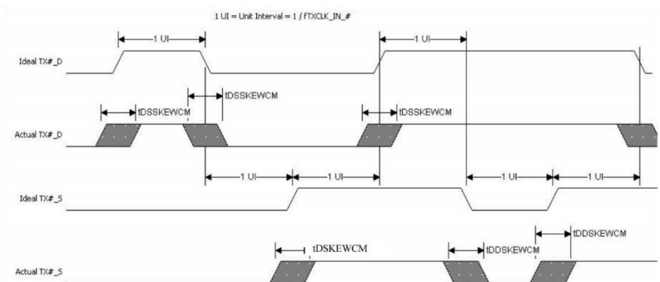
Figure 29: LVCMOS Transmit Port Data/Strobe Output Skew
