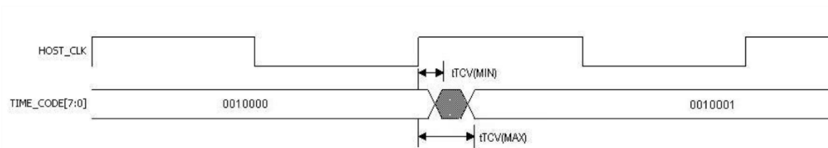
Figure 34: HOST_CLK to TIME_CODE Transition
