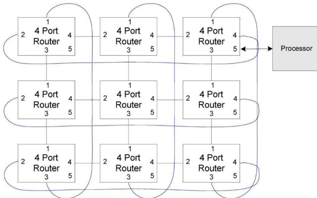
Figure 18: Distributed Network Example #1
