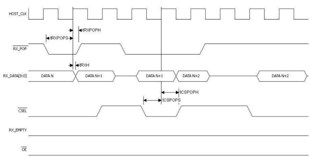
Figure 39: Receive Port POP
