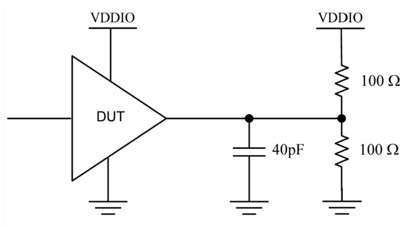
Figure 28: CMOS Equivalent Test Load
