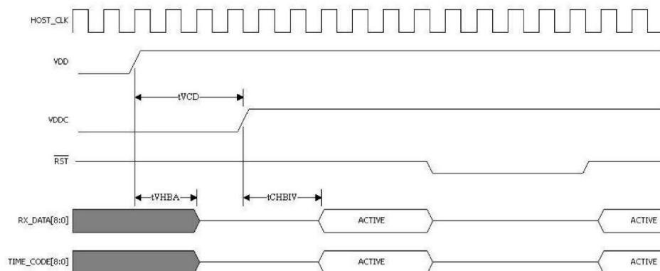
Figure 20: Power Sequencing and Reset Timing Diagram
