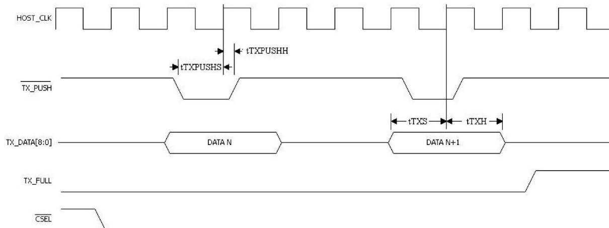
Figure 36:Transmit Port PUSH
