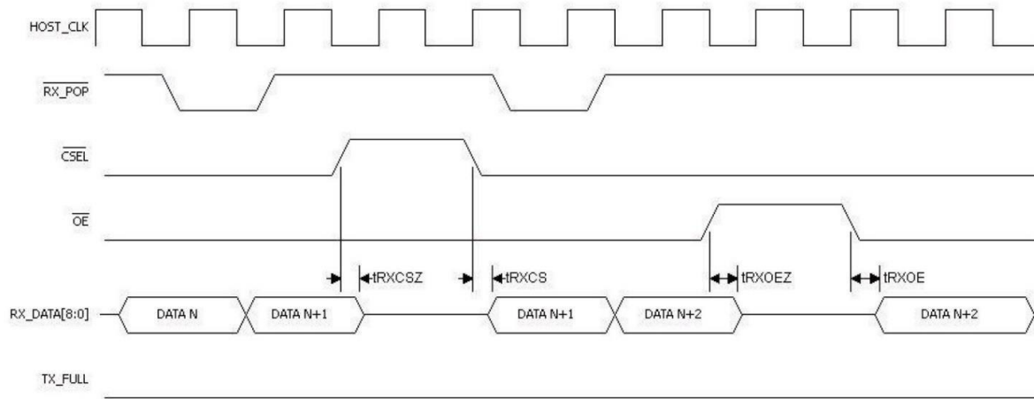
Figure 41: Control Inputs Timing Information
