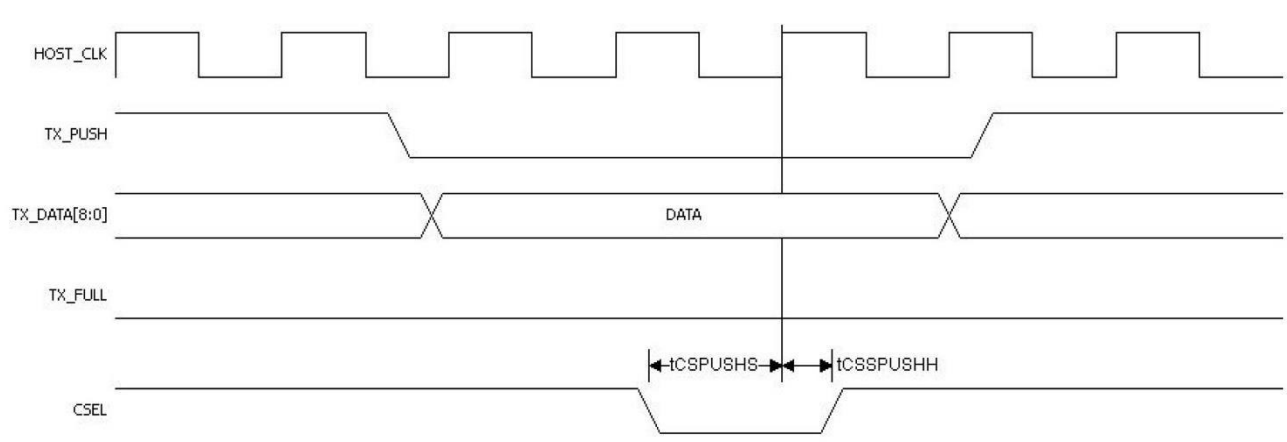
Figure 37:Transmit Port PUSH with Chip Select Transition
