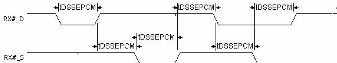
Figure 30: LVC MOS Receive Port Minimum Data/Strobe Separation
