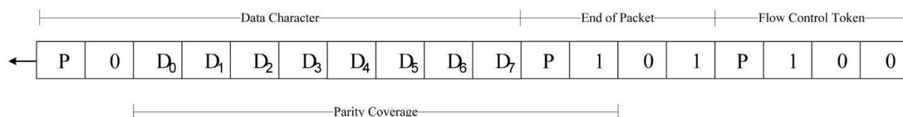
Figure 9: Parity Coverage
