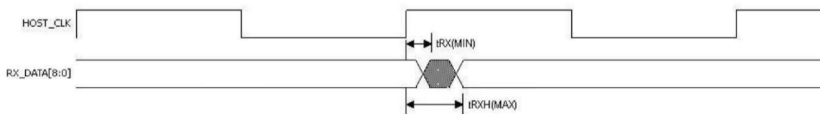
Figure 40: HOST_CLK to RX_DATA Transition
