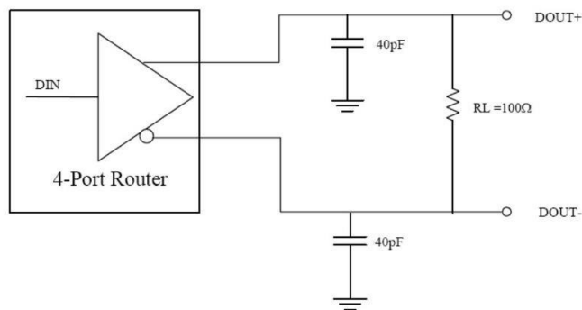
Figure 22: LVDS Driver Differential Skew, Rise and Fall Time Test Circuit
