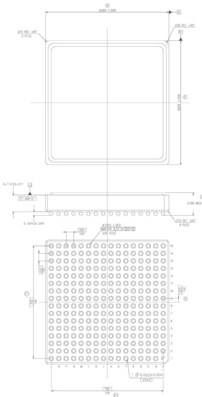
Figure 43: 255-CBGA
