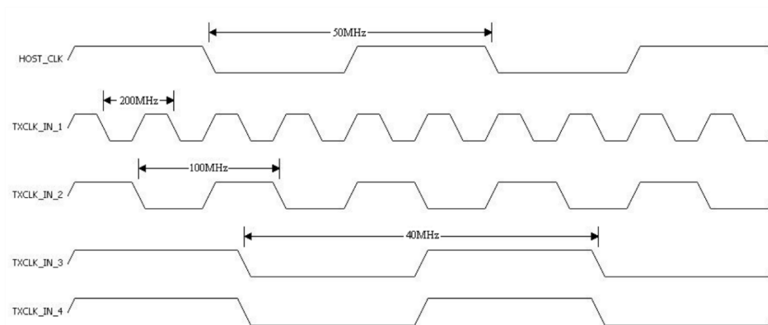
Figure 31: HOST_CLK max TXCLK_IN requirements
