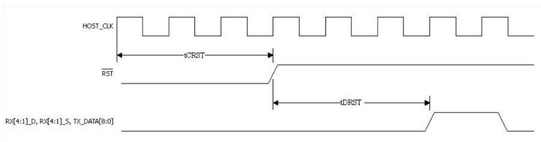
Figure 21: Reset Timing Diagram
