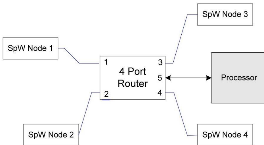
Figure 17: Centralized Network Example
