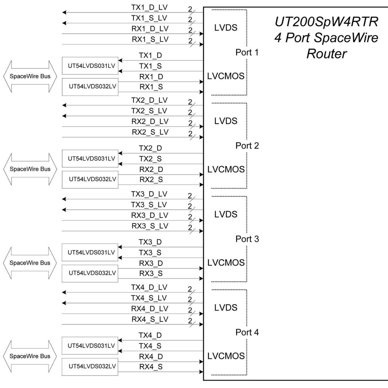
Figure 5: 4-Port Router External LVDS Interface
