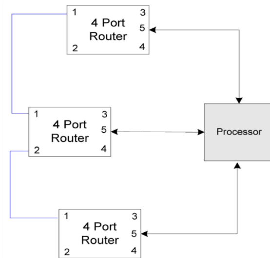
Figure 16: 8-Port Extended Configuration Using uP
