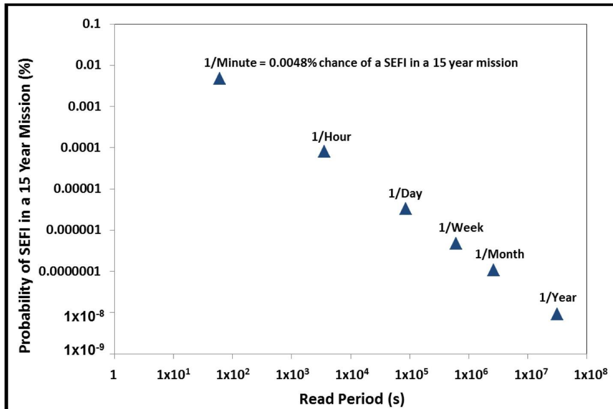
Figure 3: SEFI Probability vs Read Period
