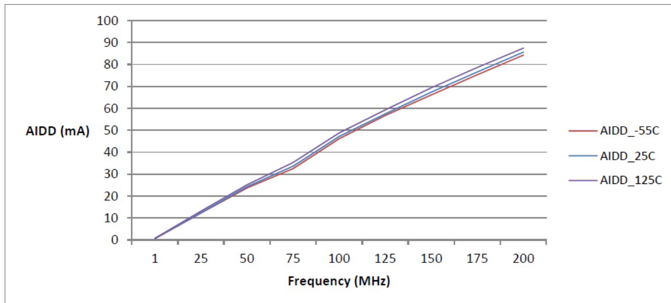
Figure 1.1 UT54ALVC2525 Characterization Plots: AIDD vs. Frequency
