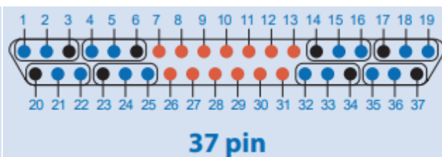
J1 and J2 Connector Pin Orientation for the 25-Pin and 37-Pin RPS Front Panel Connectors (View from the Front of the Card)
