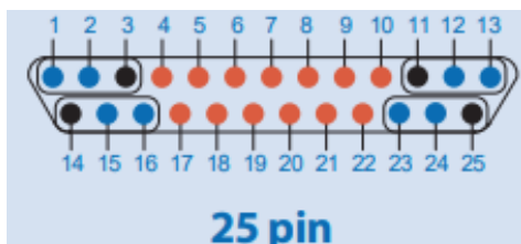
J1 and J2 Connector Pin Orientation for the 25-Pin and 37-Pin RPS Front Panel Connectors (View from the Front of the Card)
