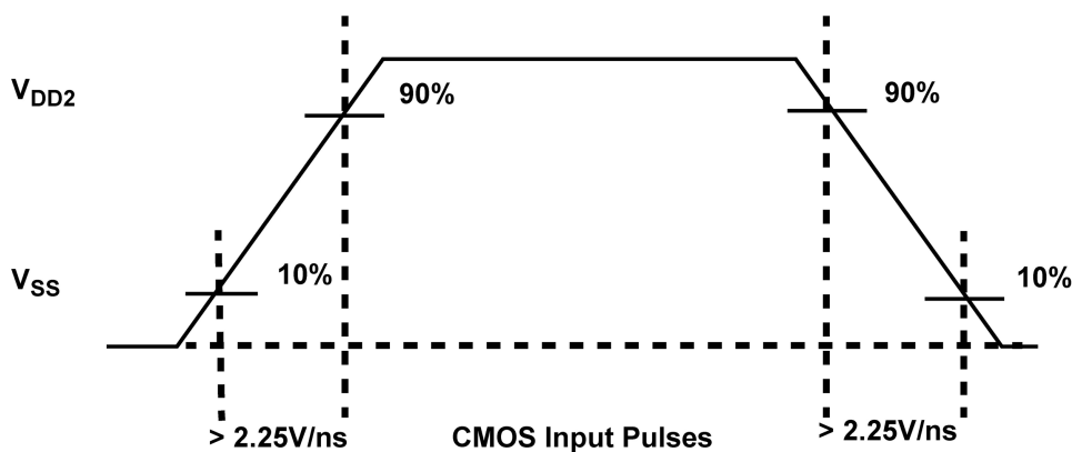
Figure 8. AC Test Loads and Input Waveforms
