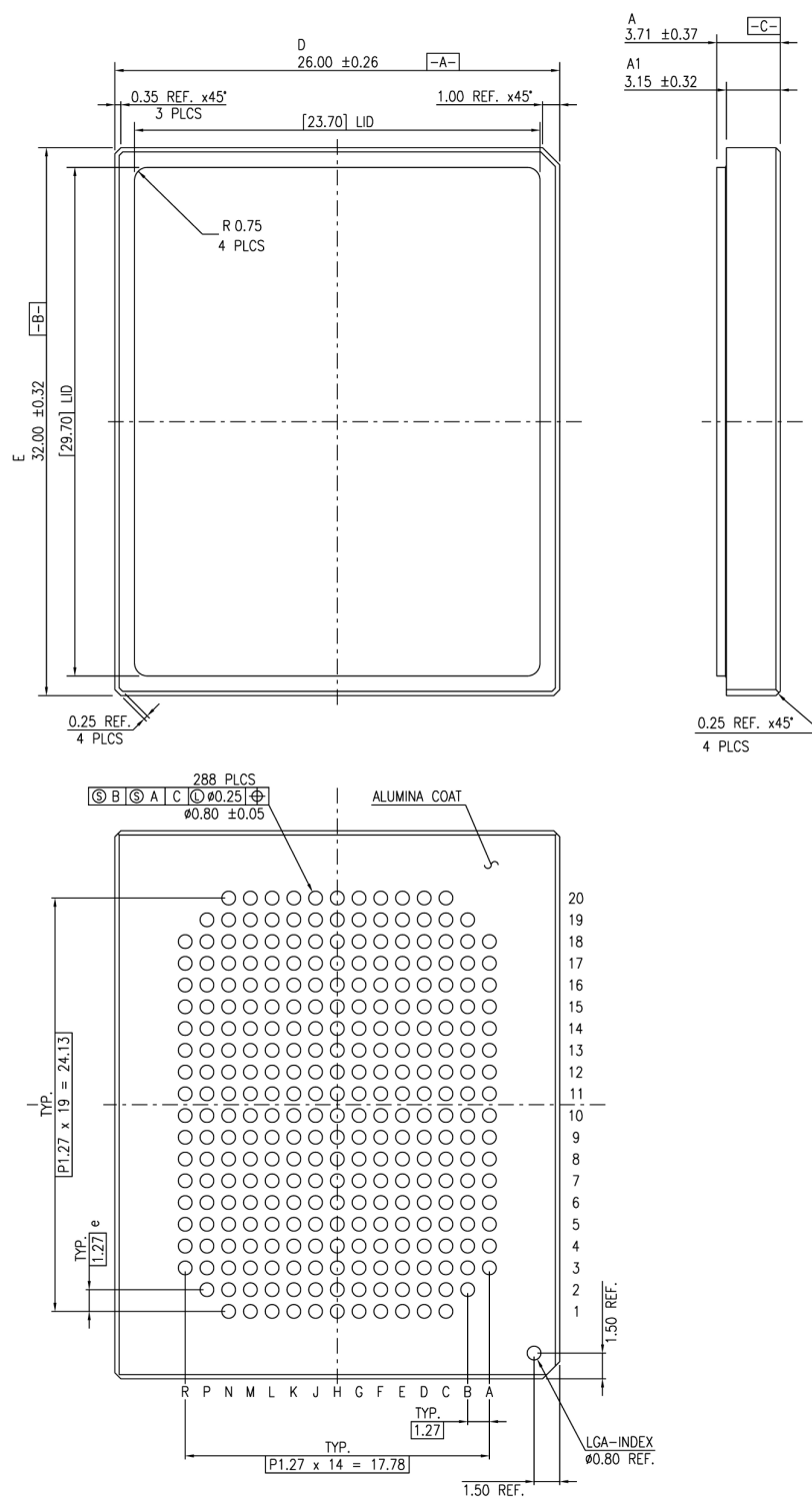
Figure 10. 288-Lead CLGA
