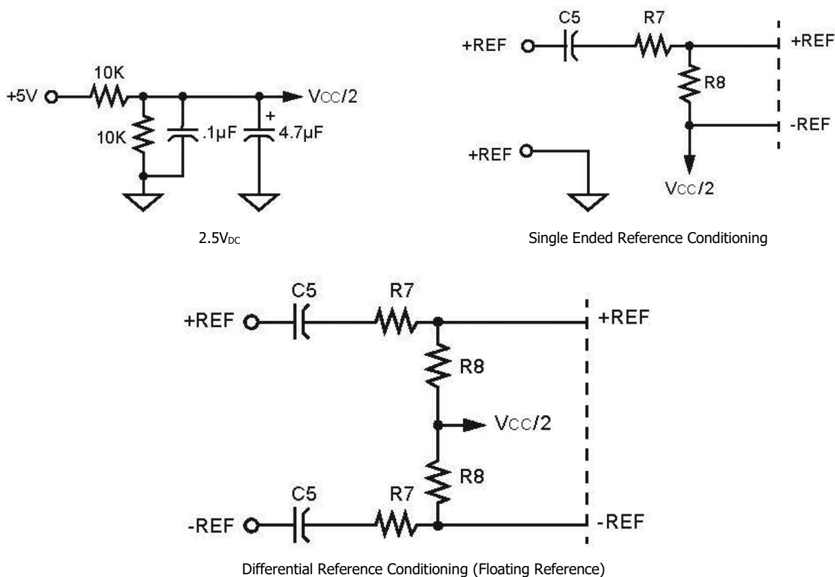
Figure 5: RDC5028 Resolver, Synchro and Reference Input Configurations
