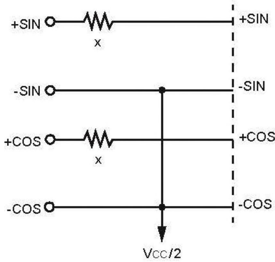
Direct Resolver
