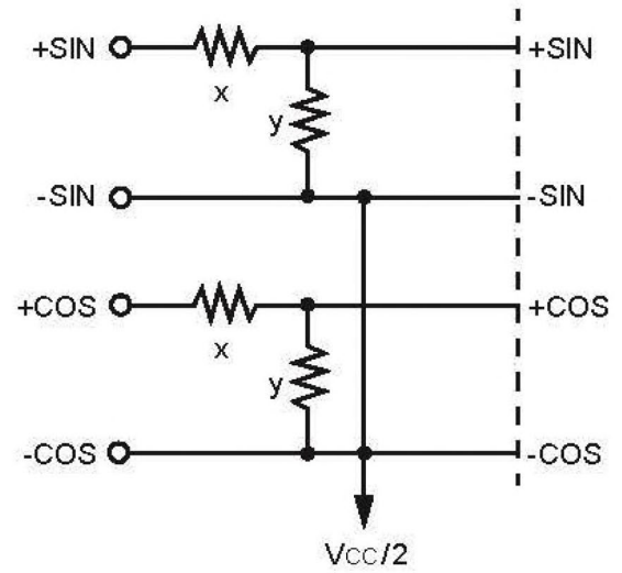
Single Ended Resolver Conditioning
