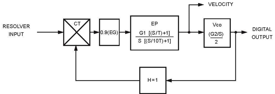
Figure 4: RDC5028 Transfer Function Diagram
