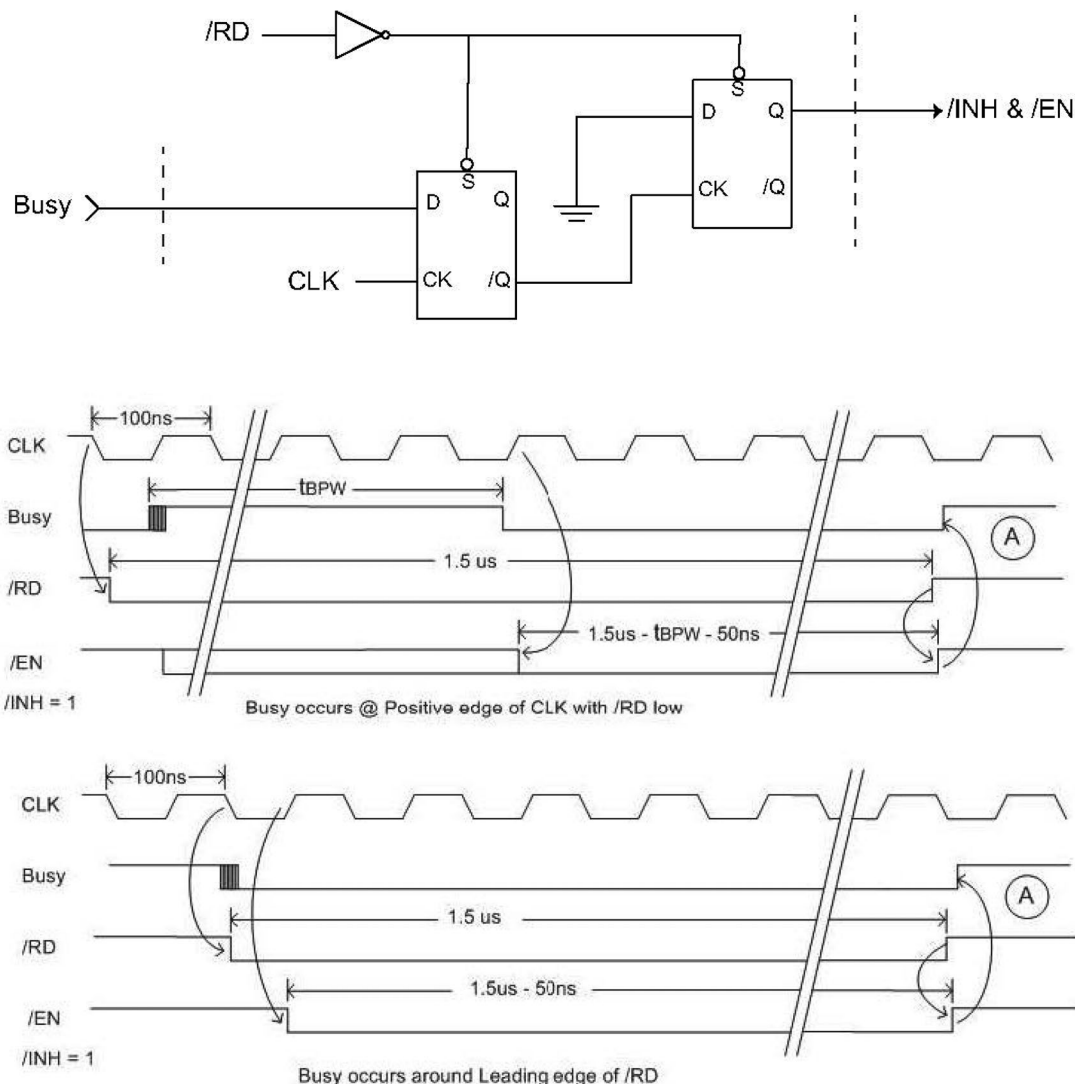
Figure 6: Circuit Timing Waveforms
