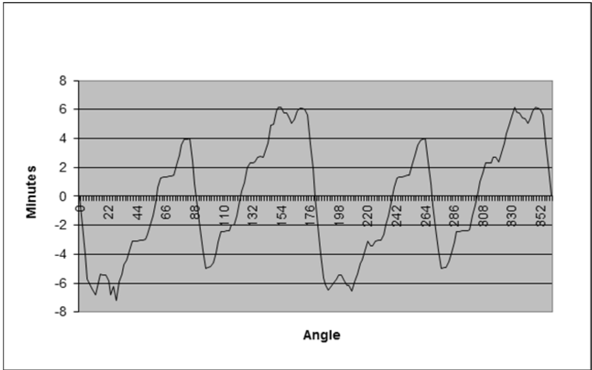
Figure 9: Angle Error Chart 5028-3-2
