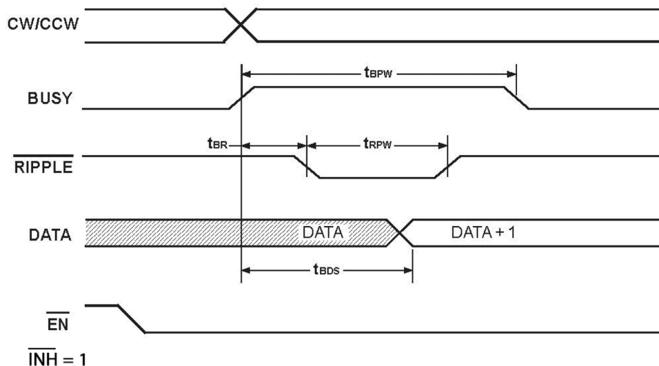
Figure 2: RDC5028 Timing Diagrams
