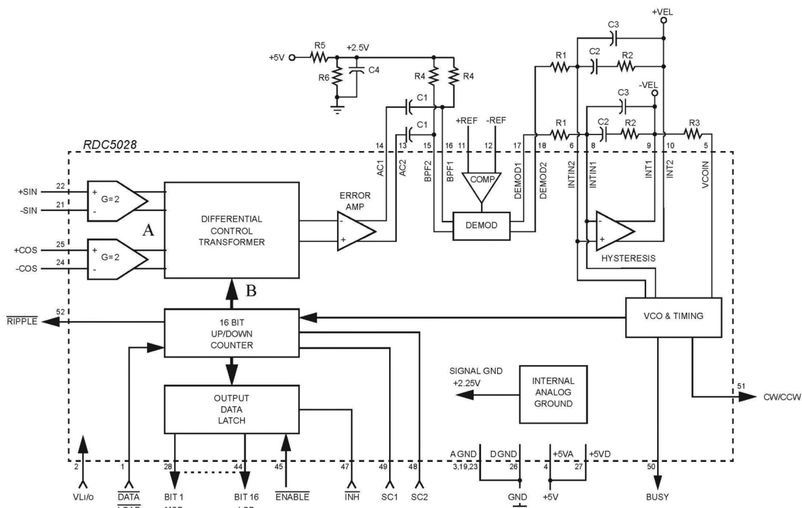
Figure 1: RDC5028 Block Diagram
