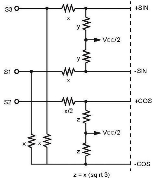
Synchro Conditioning
