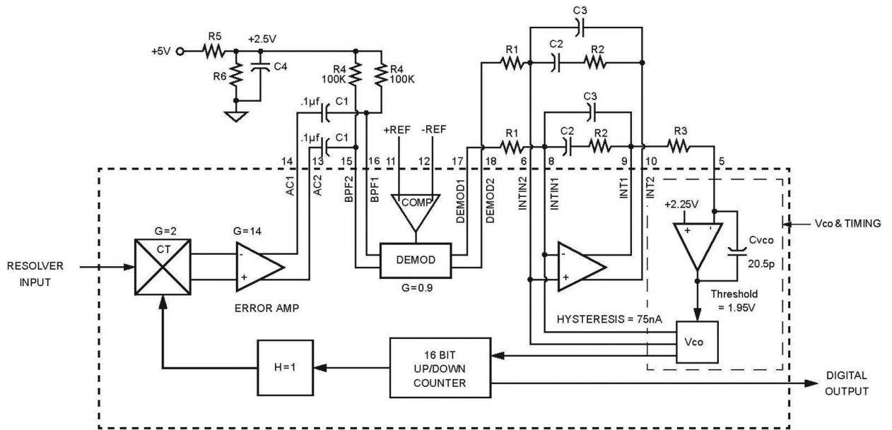
Figure 3: RDC5028 Functional Block Diagram
