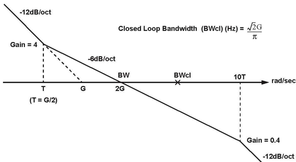
Figure 5: RDC5028 Open Loop Bode Plot
