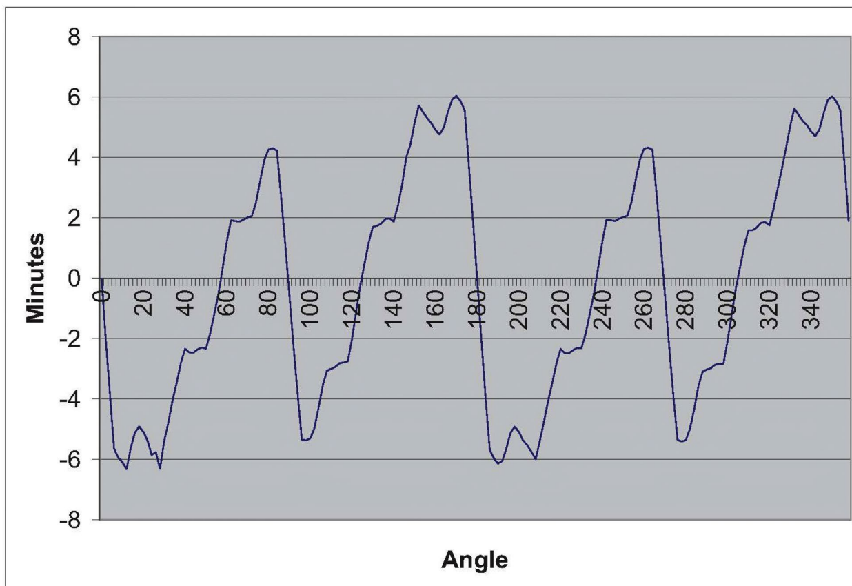
Figure 8: Angle error chart 5028-3-1
