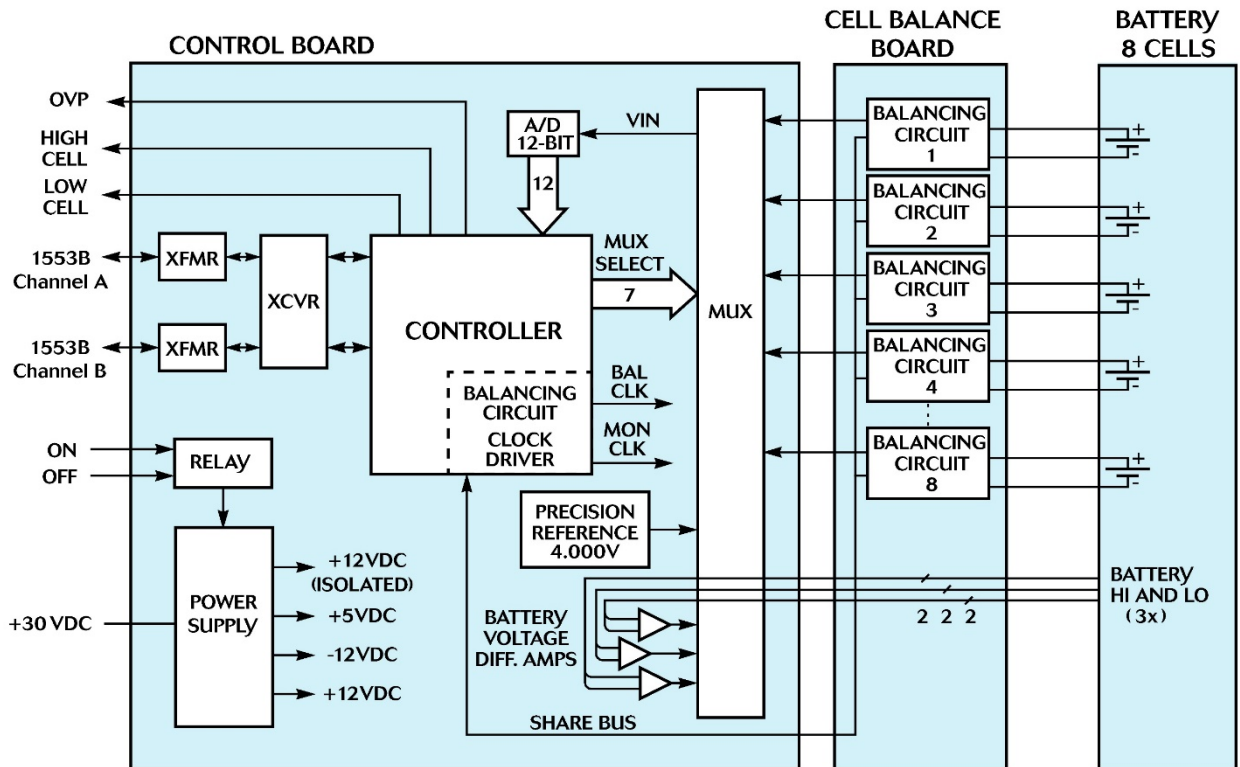
Block Diagram
