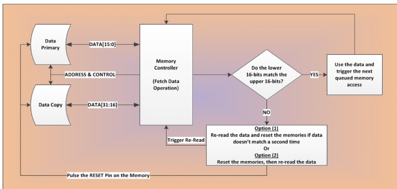
Figure 5: Memory Redundancy Flow Diagram
