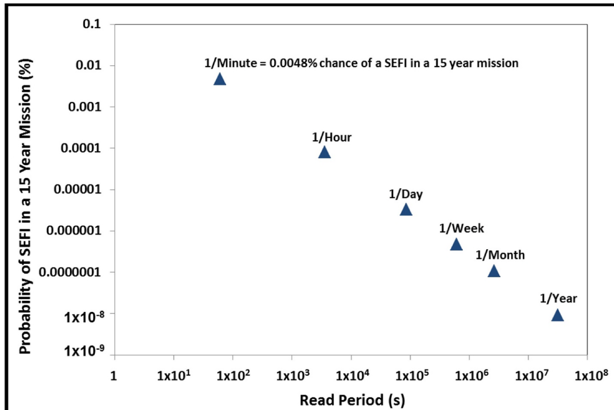
Figure 3: SEFI Probably vs Read Period
