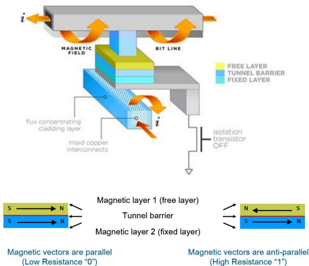
Figure 1: Cross-section diagram of the MRAM memory cell
