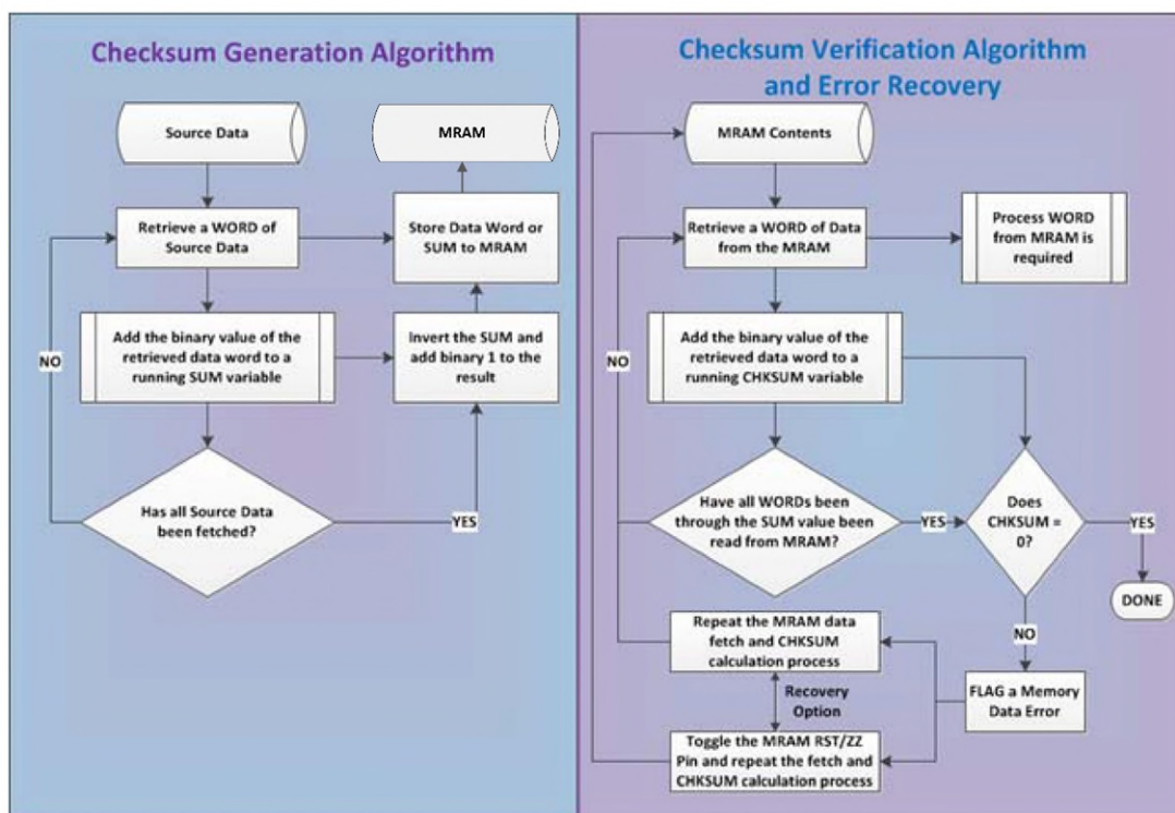
Figure 4: Modular Checksum Generation and Verification Algorithm Flow Charts
